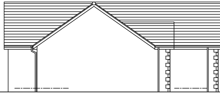
Side (garage) Elevation
